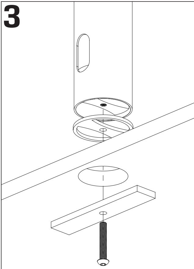
FOR BUSHING
