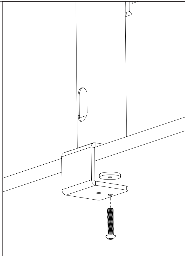
FOR CLAMP
